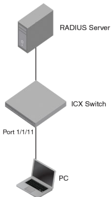
FIGURE 20 802.1X authentication or MAC authentication with dynamic ACL assignment
