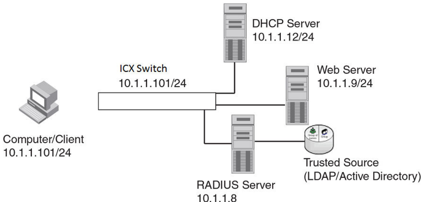
FIGURE 29 Basic topology for web authentication
