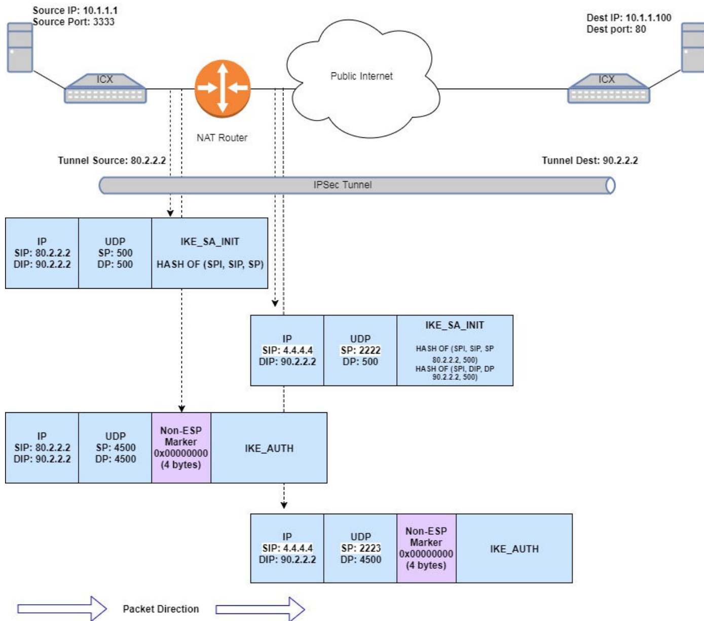
FIGURE 24 IPsec over NAT- Control flow
